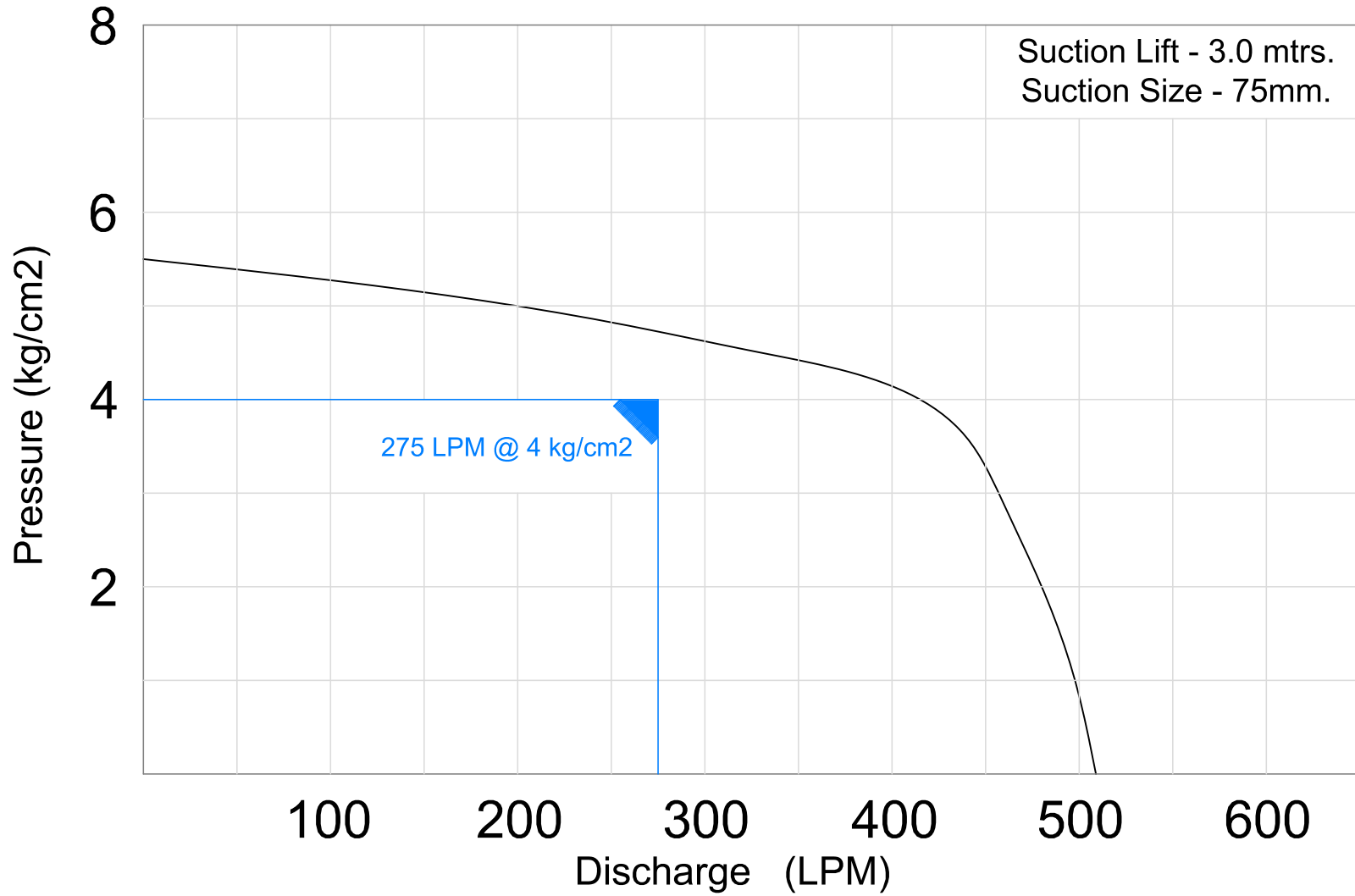
Typical Performance of MFP 275 D-M
